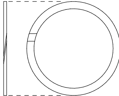
TEFLON BACK LIP P/N P11227-219 REPLACES P/N 12-8774T024 QTY: 2
