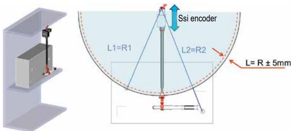
1 encoder system
