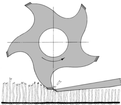
Mobile Teppichschermaschine TS 120 U Mobile Carpet shearing machine TS 120 U
