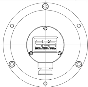
SB-2550-L EXTERNAL BALANCER: 114mm STD-CABLE
