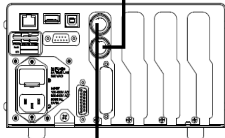
SB-5501 CONTROL: MECH, AC INPUT, NO PROFIBUS
